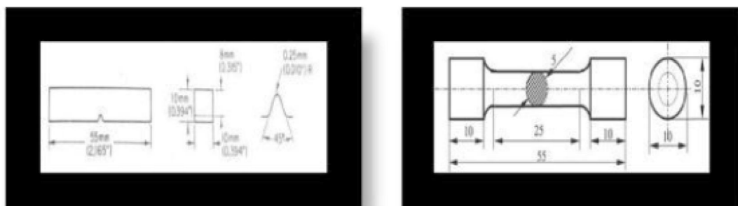
Fig.3. (a) Dimensions for Charpy test sample (b) Dimensions for UTS test sample
