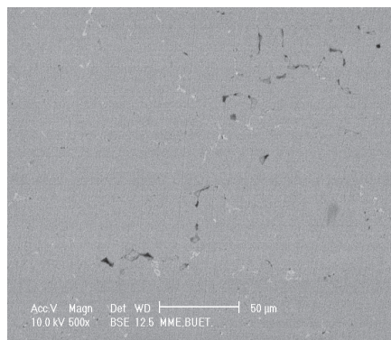
Fig. 7(c). BSE image of plate 3
