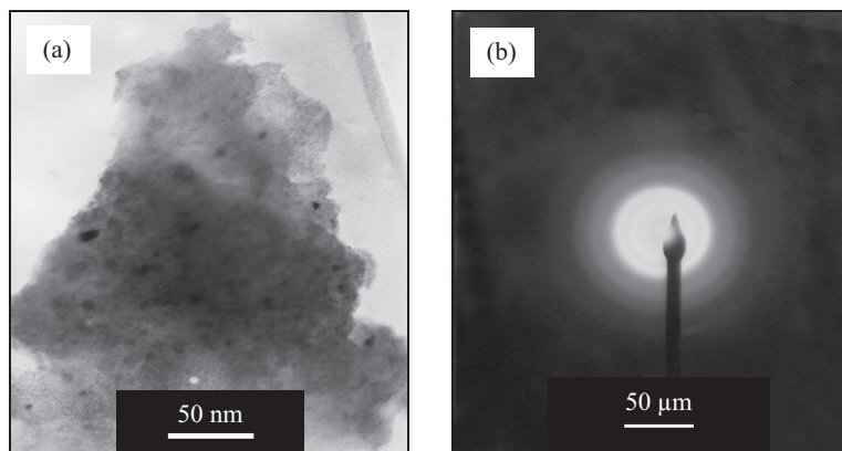
Fig. 2. TEM image of \text{Mg}_2\text{Ni} alloy: (a) light-field image (b) electron diffraction pattern.
