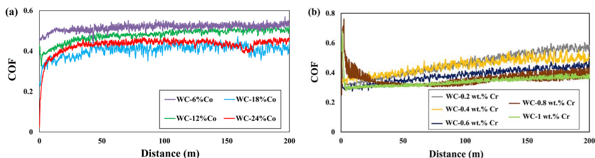
Fig. 11. COF-distance diagrams of the studied cermet: a) WC-Co and b) WC-Cr
