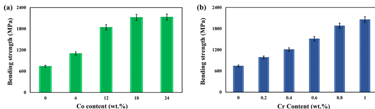
Fig. 10. Bending strength values of the SPS-ed cermet containing different contents of the binders: a) WC-Co and b) WC-Cr
