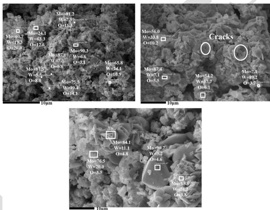
Fig 12- EDAX analysis of the reduced sample MoO 3 -26.5wt% WO 3 at 800°C
