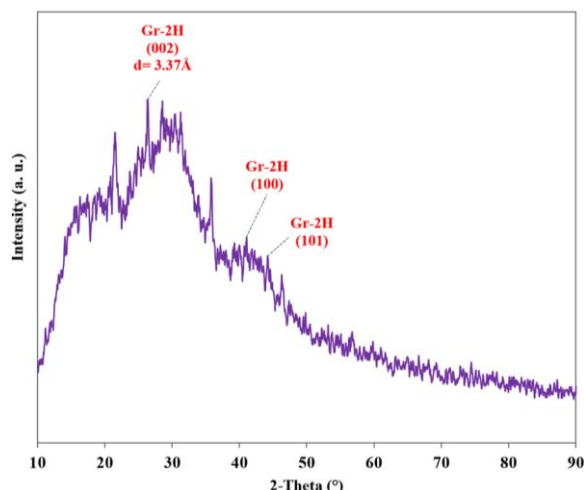
Fig. 2. XRD pattern of GCNP sample representing indicating the composite nature of the material consisting of crystalline and amorphous phases. The inset shows the comparison of the sample peaks with Graphite-2H (PDF 41-1487) which matches to a high extent
