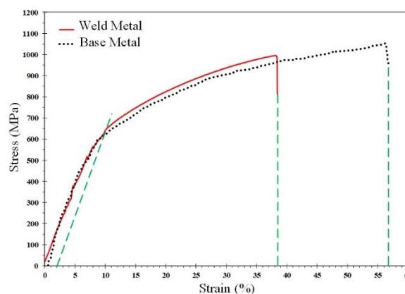
Fig. 6. Room temperature stress-strain graph of base metal and weld metal of the optimal welded sample
