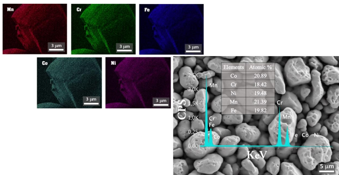
Fig. 4. EDS analysis of the powders after MA
