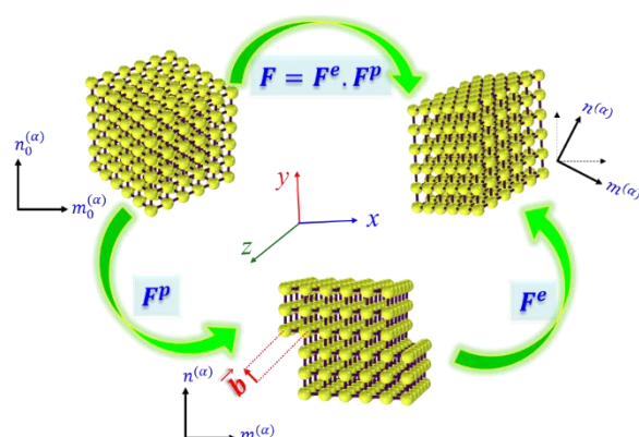
Fig. 2. The hypothesis of crystal plasticity's deformation gradient, F = F^e . F^p
