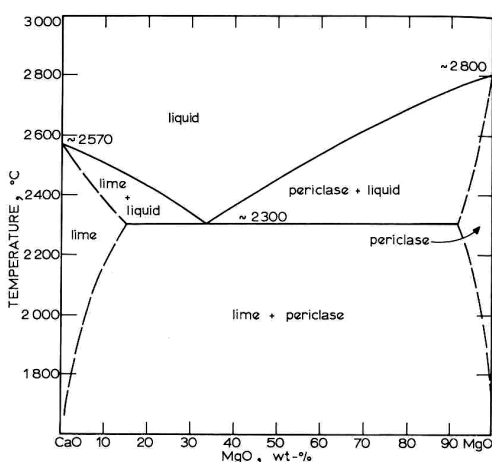
Fig. 1. The MgO- CaO system [3].
