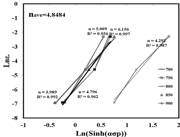
Fig. 7- The relationship between \ln(\dot{\epsilon}) - \ln[\sinh(\alpha\sigma)] .
