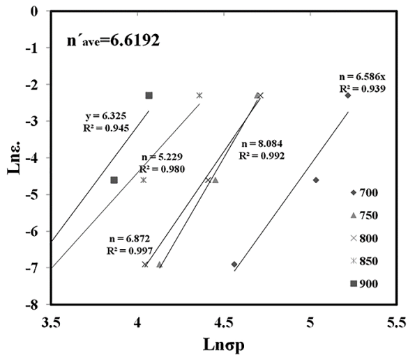
Fig. 6- The relationship between \ln(\dot{\epsilon}) - \ln(\sigma) .
