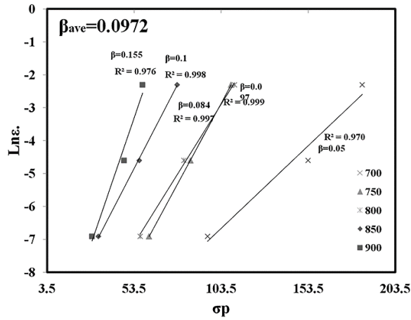
Fig. 5- The relationship between \ln(\dot{\epsilon}) - \sigma .
