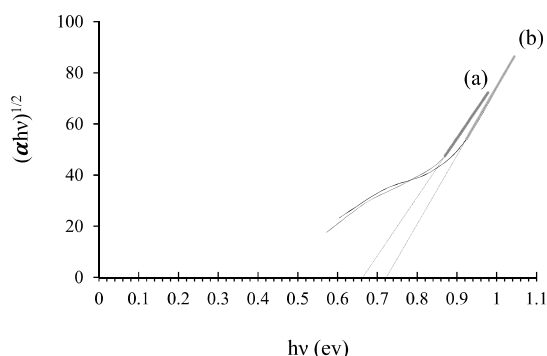
Fig. 4. The (\alpha hv)^{1/2} versus h\nu plotted for \text{Ge}_{1-x}\text{C}_x coating: (a) \text{R}_1 and (b) \text{R}_2 .
