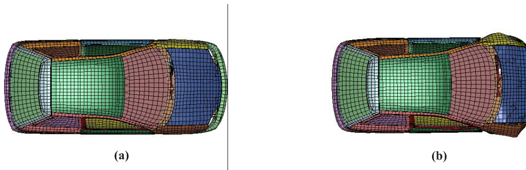
Fig. 2. Crash model of the vehicle (Top View); (a) Undeformed, (b) Deformed (80 ms)
