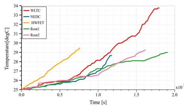
Figure 10: Comparison of battery temperature changes over time under five different driving cycles.
