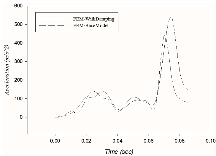
Fig18. Effects of the structural damping on time history of the acceleration of the occupant's body
