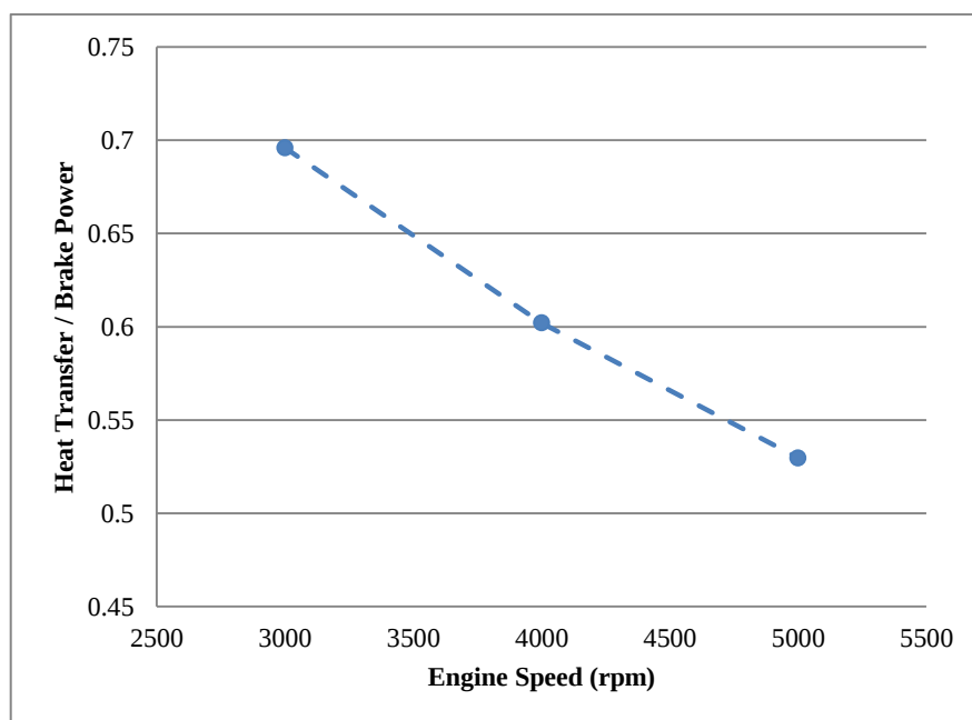
Fig.12. Heat Transfer to Brake Power Ratio
