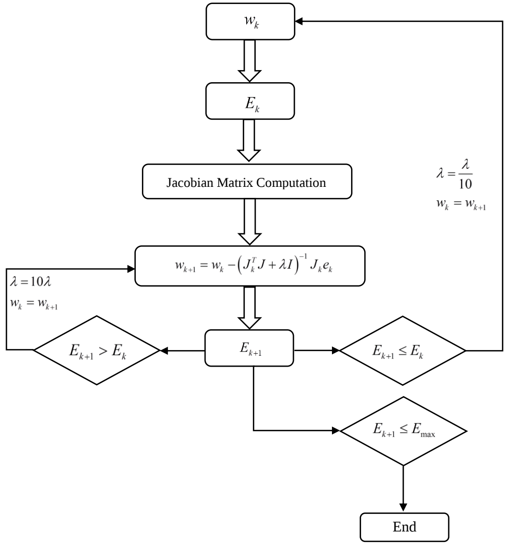
Fig. 2. Block-diagram for training using Levenberg-Mardquardt algorithm; W_k is the current weight, W_{k+1} is the next weight, E_k is the current total error and E_{k+1} is the next total error.
