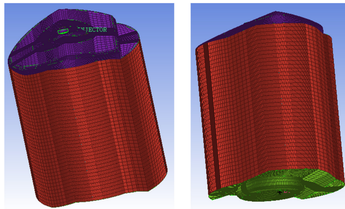
Fig1. Engine mesh generated in ICEM-CFD
