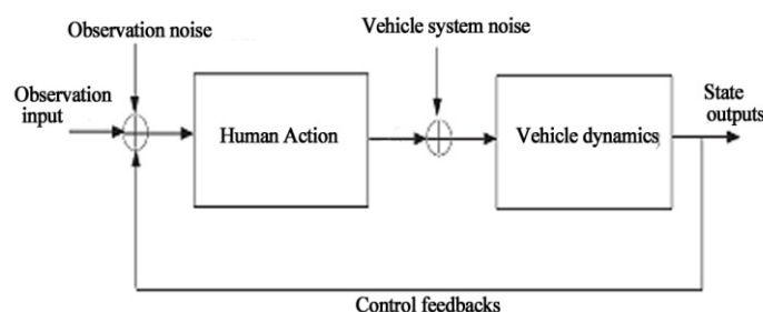
Fig3. Structure of a DVU model [2].
