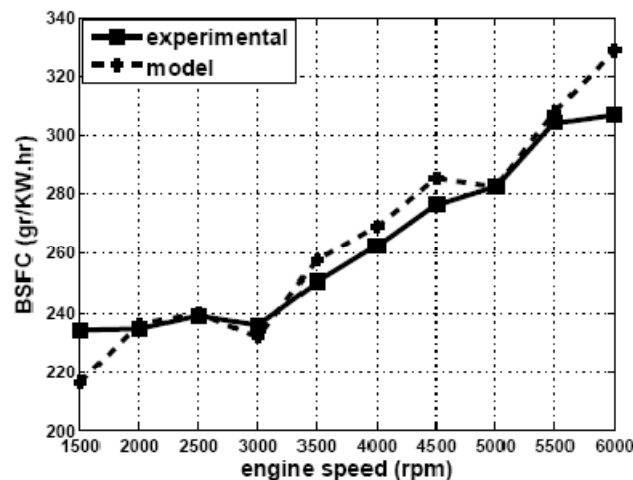
Fig2. validation the brake specific fuel consumption results of simulation and experimental
